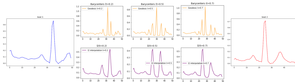
Figure 12: The difference between perturbation along the Wasserstein geodesic and on l_2 space. The geodesic perturbation keeps the structure of ECG beats while l_2 interpolation leads to situations that violates common senses (two QRS waves in one beat).
